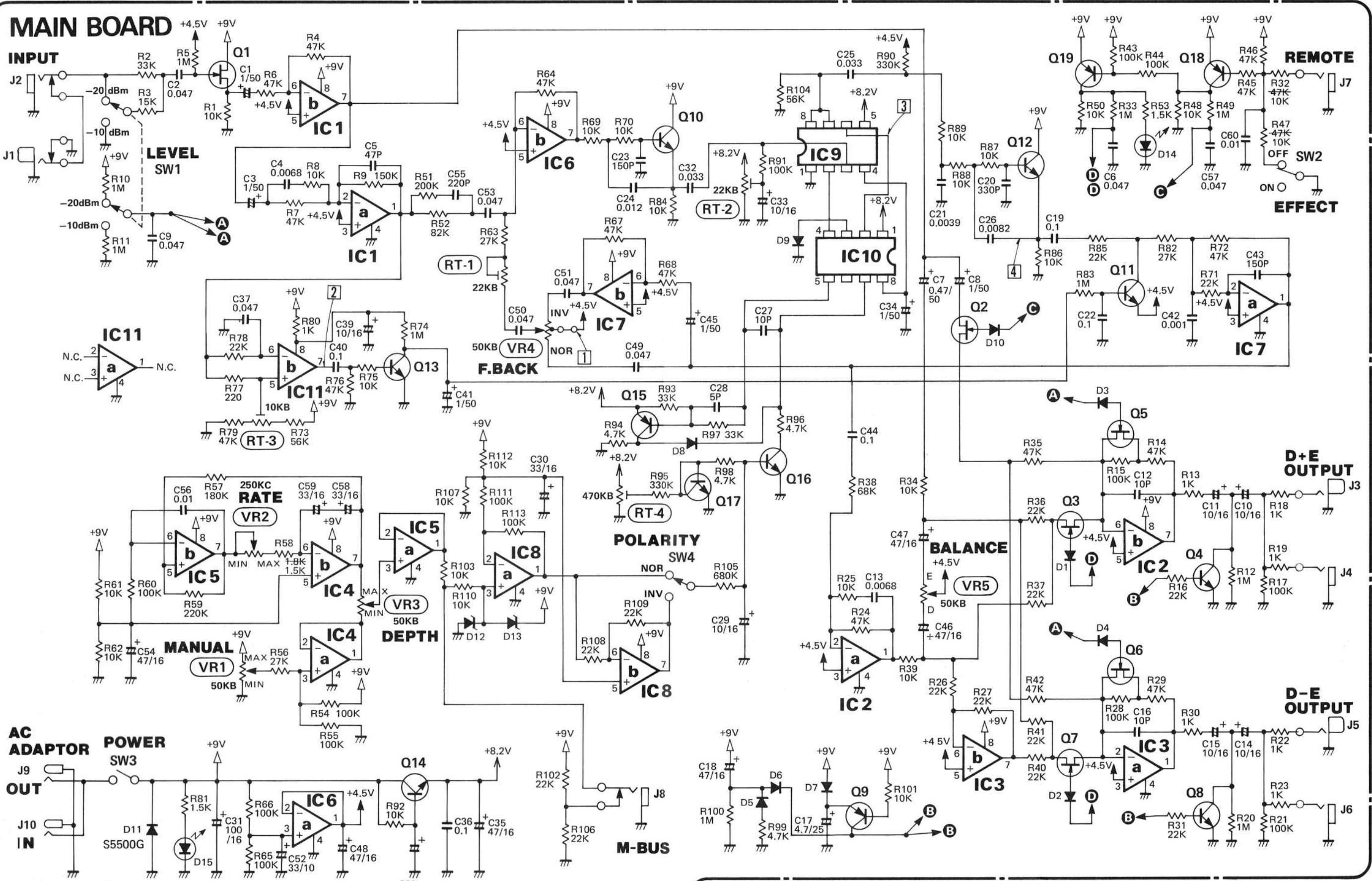
RBF-10 CIRCUIT DIAGRAM
