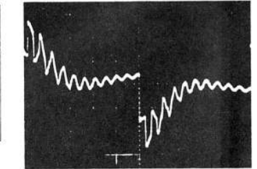
100mV/div, 2ms/div
