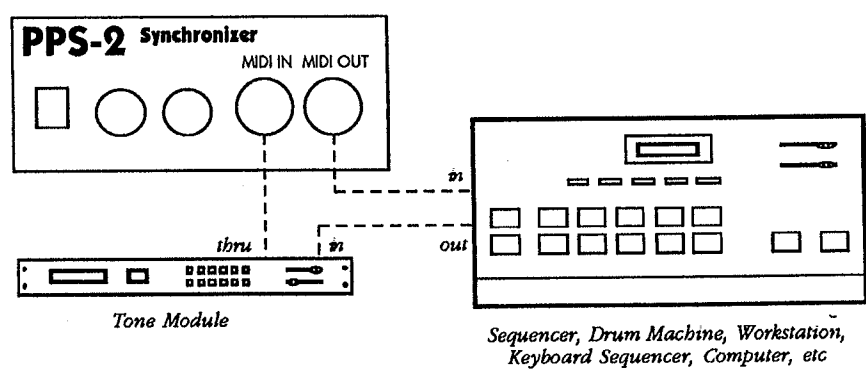
FIGURE 3: MIDI HOOK UP, NO MIDI PATCH BAY OR THRU BOX Striping and Syncing to tape while monitoring the playback of a single MIDI sound module
