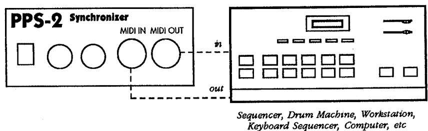
FIGURE 2: MIDI HOOK UP, NO MIDI PATCH BAY OR THRU BOX Striping and Syncing to tape
