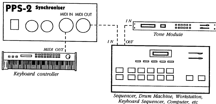
FIGURE 5: MIDI HOOK UP, NO MIDI PATCH BAY OR THRU BOX
