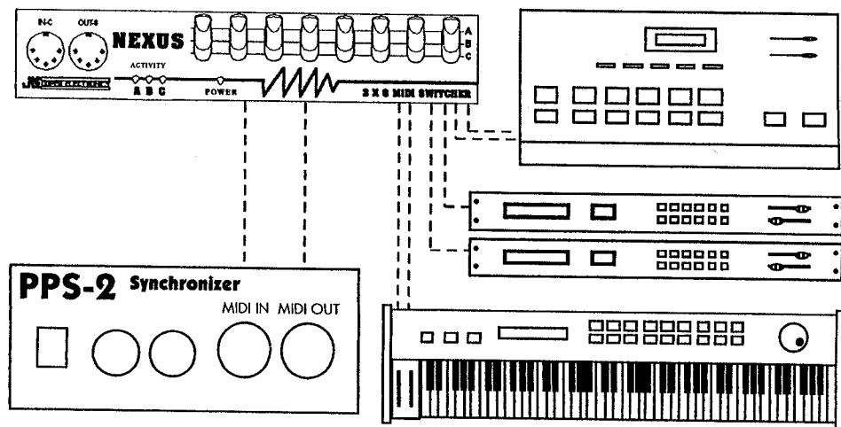
FIGURE 4: MIDI HOOK UP, WITH MIDI PATCH BAY OR THRU BOX
